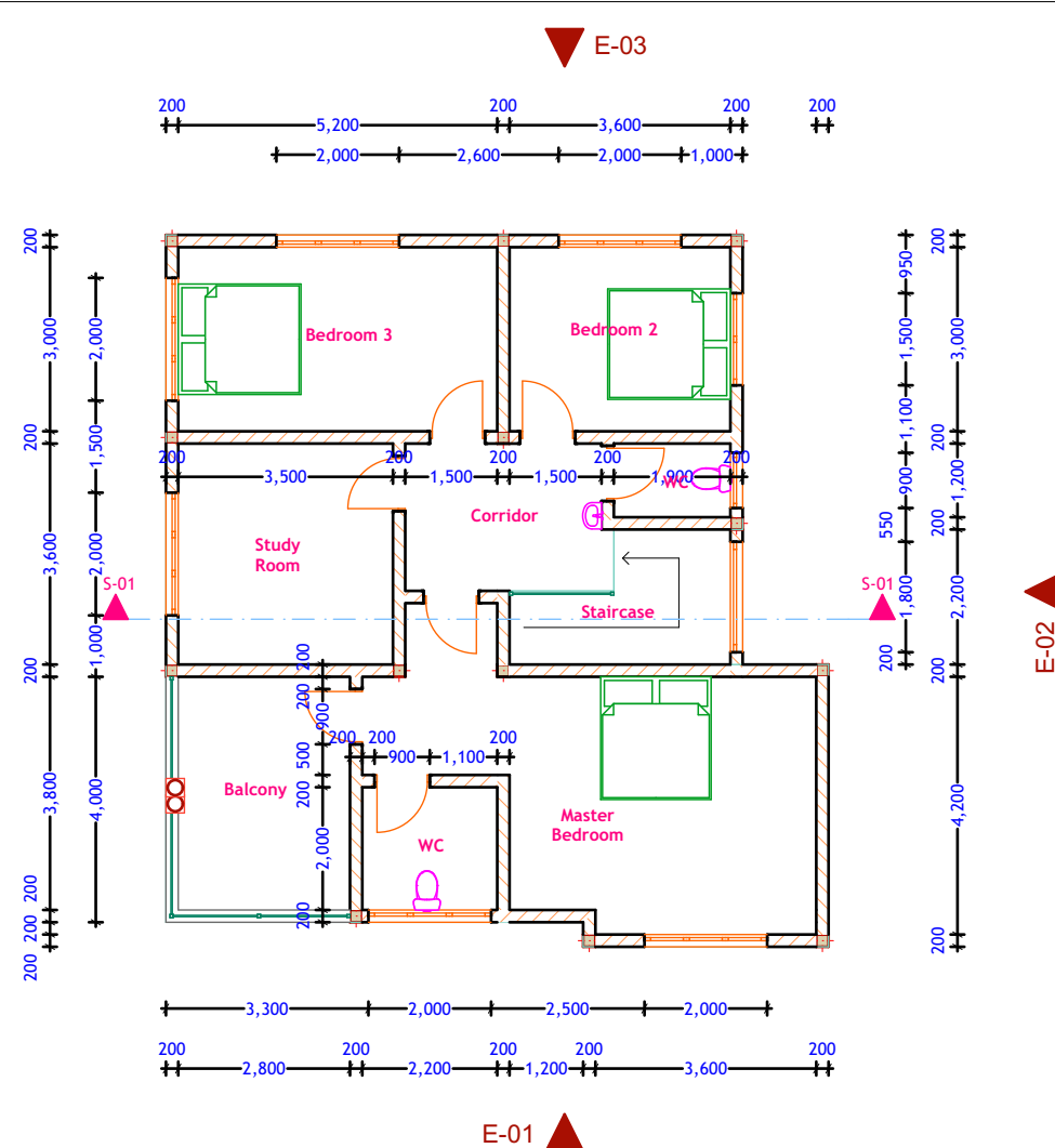
1ST FLOOR LAYOUT
